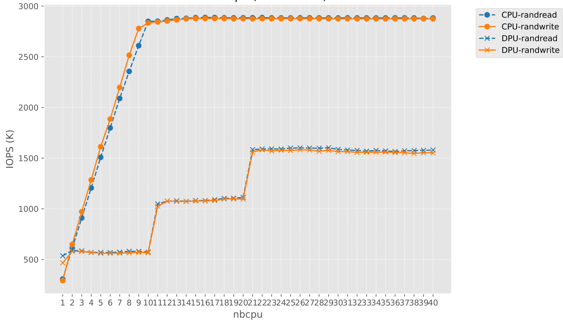
IOPS vs nbcpu (CPU vs DPU)
